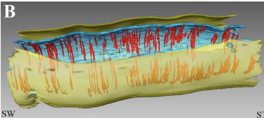
Overexpression of stable mutant FtsZ
