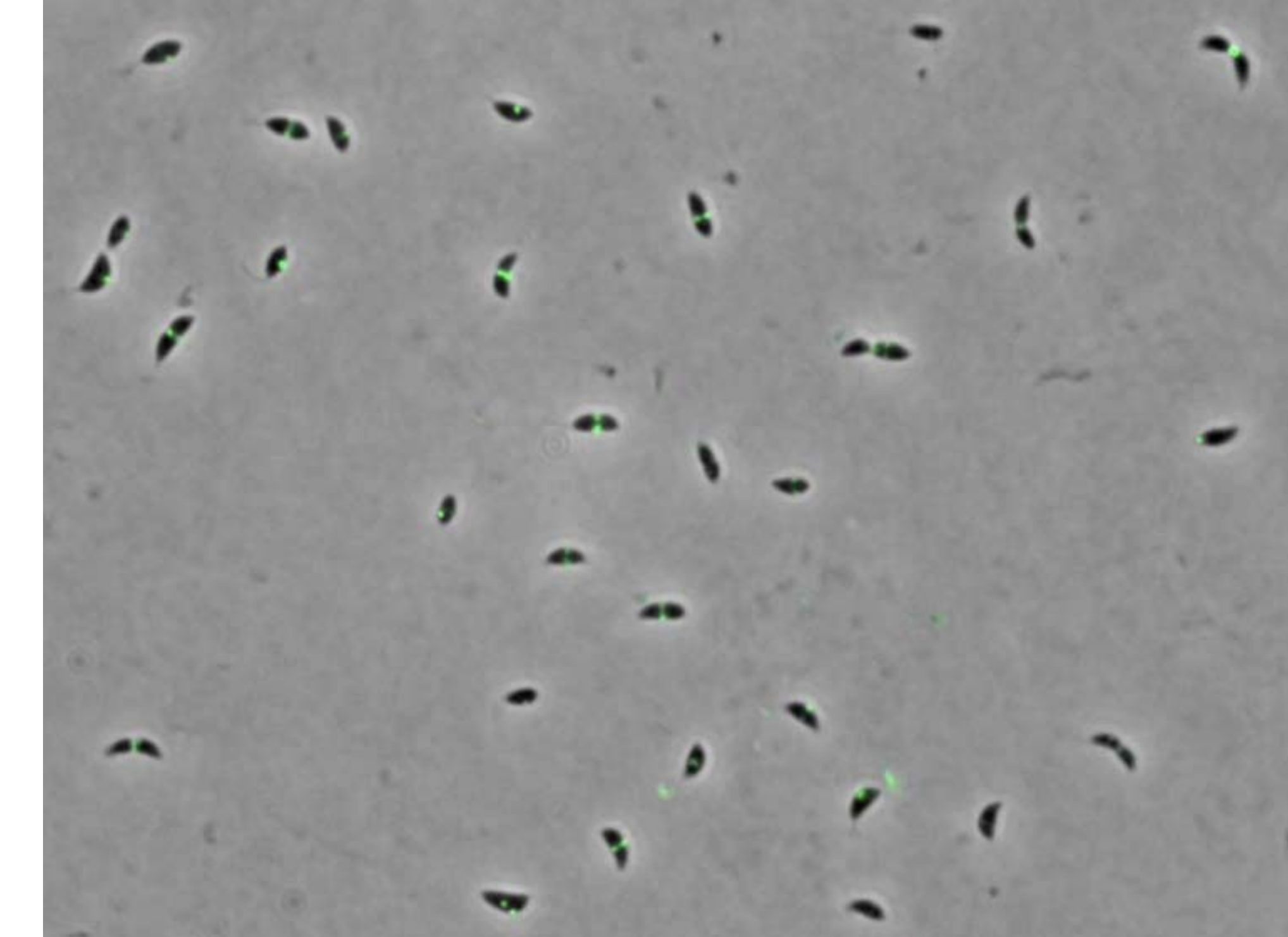
Caulobacter crescentus ftsZ-yfp
